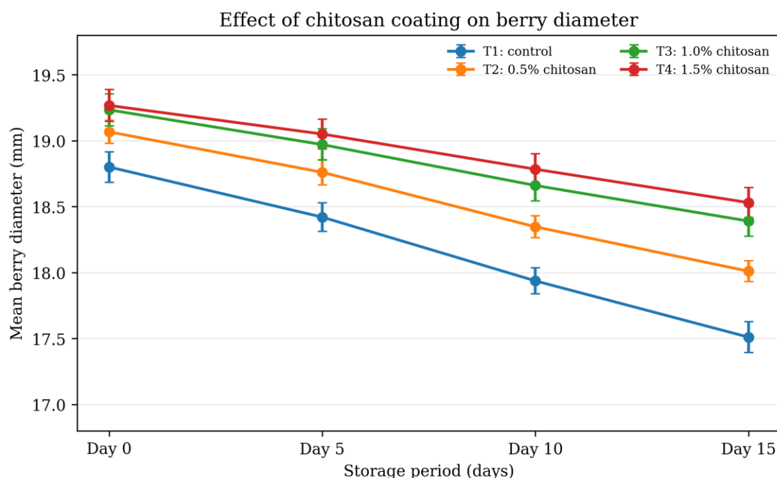
Figure 4.2: Mean berry diameter during 15 days of ambient storage. Error bars represent \pm SE (n = 3).
