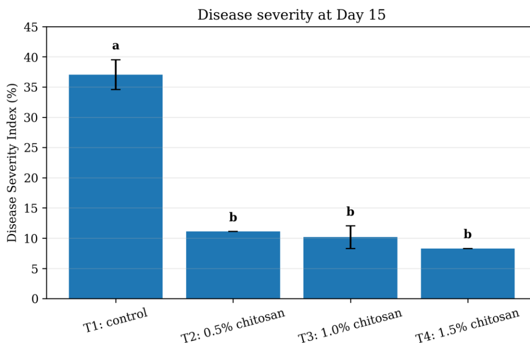
Figure 4.4: Disease Severity Index of blueberries at Day 15. Error bars represent \pm SE (n = 3). Bars with different letters differ significantly at P \leq 0.05 .
