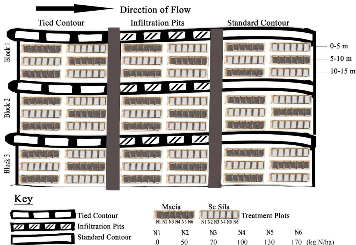
Figure 2. Experimental layout.
